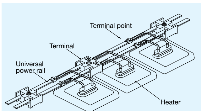
Figure 13: Rail wiring
