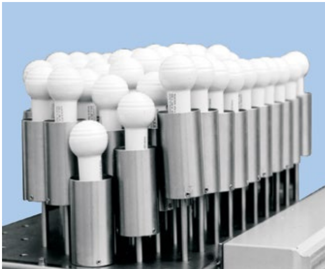
Figure 8: 3-D heating panel for laminating door trims
